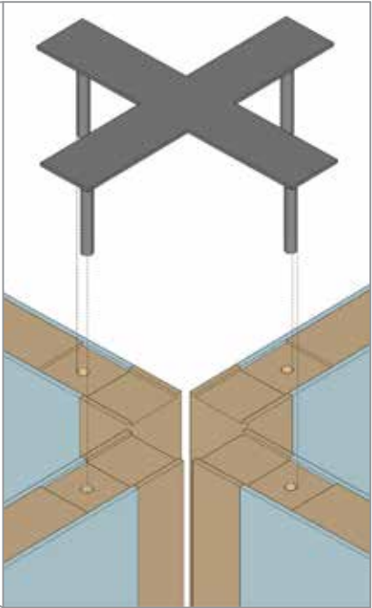
DETALLE GRAPA
